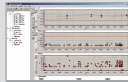
Data alignment
